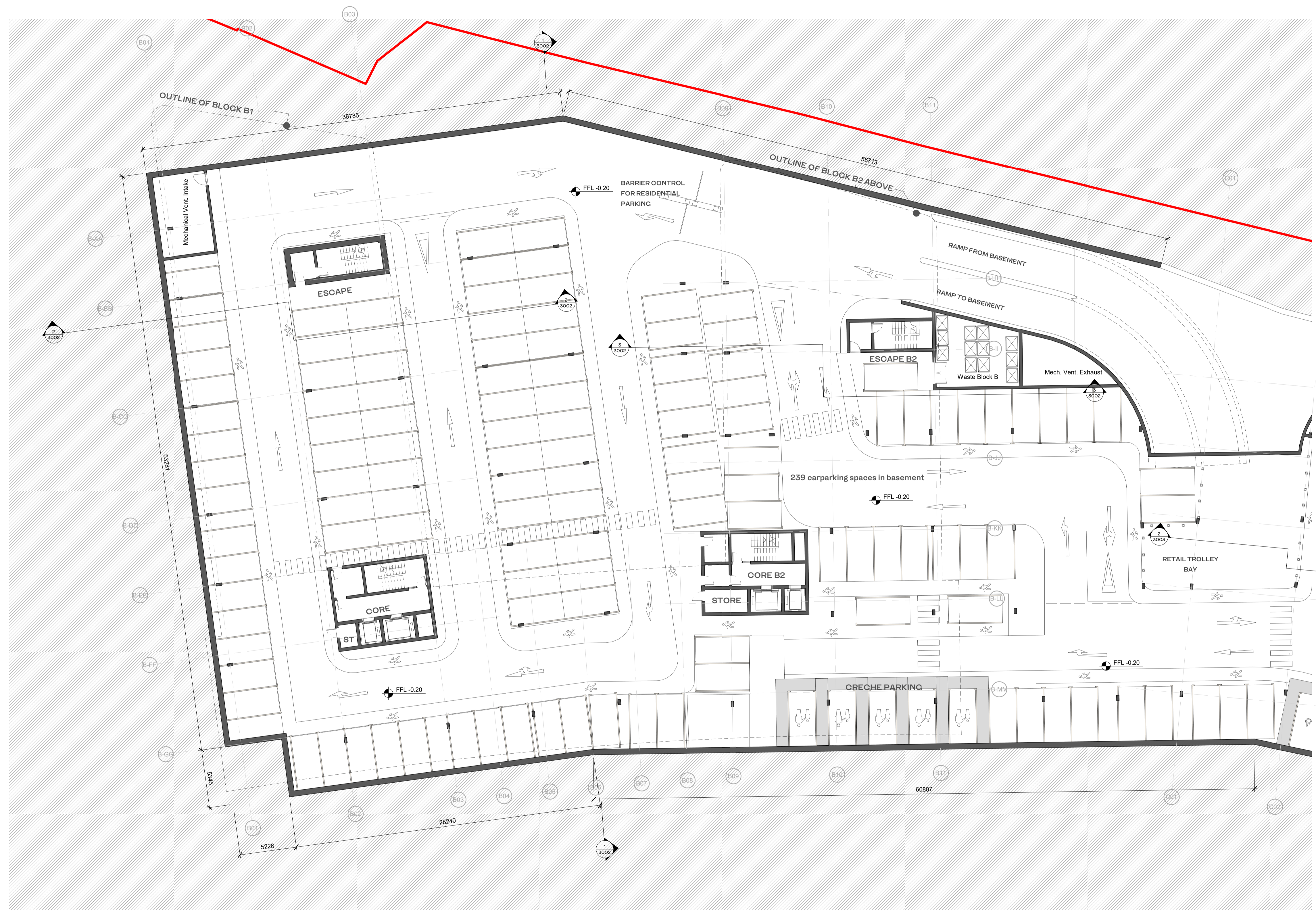
1 ZONE 02 - BLOCK B - B01 BASEMENT 1:200
